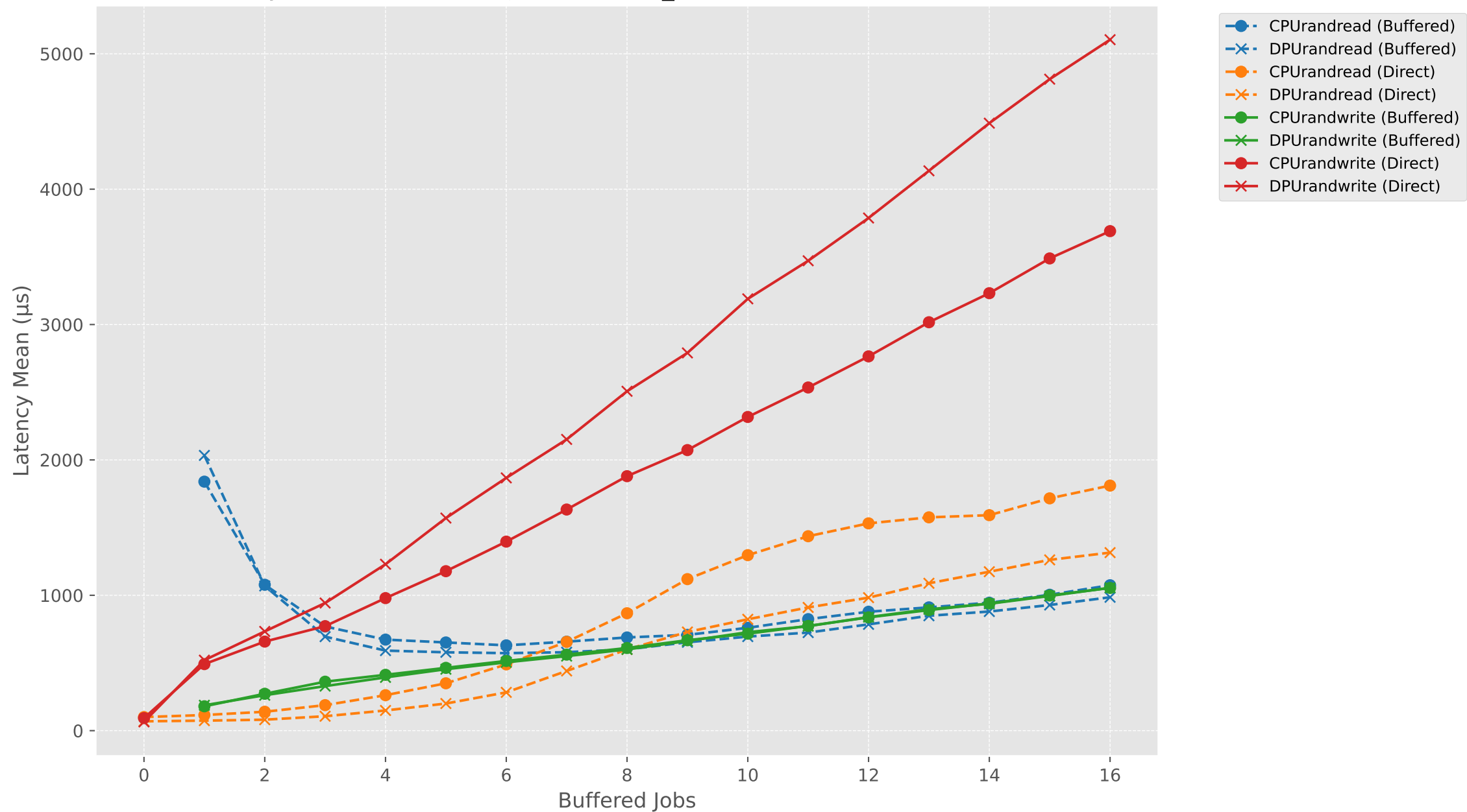
Latency Mean vs Buffered Jobs (direct1_bufferedN) - RAND (CPU vs DPU)
